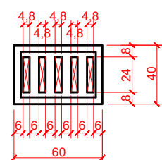
N1-2Ø3/8 C=55 N2-6Ø3/8 C=35
